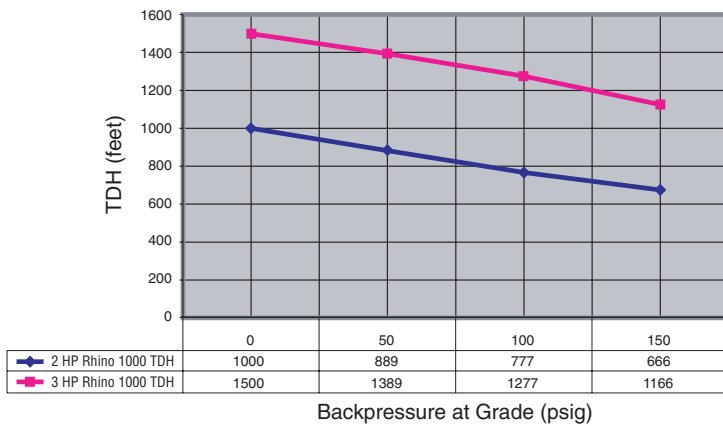
Rhino MiniJack 1000 TDH Vs. Backpressure
